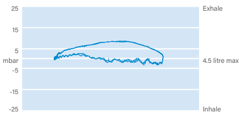
Breathing effort at 50 msw and 50 bar: 0.72 J/l.
