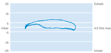
Breathing effort at 50 msw and 50 bar: 0.63 J/l.
